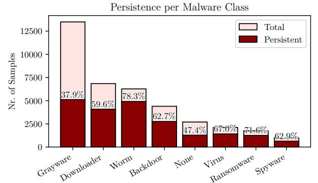
Figure 8: Persistence rate per malware class in Dataset I: Classes are labeled using AVClass [86, 87], and only those with at least 1,000 samples are shown.
