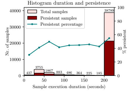
Figure 4: Execution duration vs. persistence count: Samples running under 200 seconds ended voluntarily, while those still active at 200 seconds were forcibly terminated by the sandbox.
